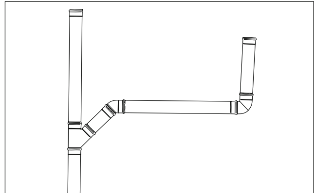
Fig. 5. Branch pipes with a minimum connection angle of 45^\circ can be used when connecting ventilated side pipes.
